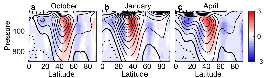
Figure 1. Zonal wind in (a) October, (b) January, and (c) April averaged for the years 1981–2014 (contours, contour intervals 5 m/s), and red and blue colors represent eddy momentum flux convergence and divergence, respectively ( \times 10^5 \text{ m}^2/\text{s}^2 ) for the zonally averaged North Pacific (longitudes 160^\circ\text{E} – 137.5^\circ\text{W} ) calculated from the National Centers for Environmental Prediction Reanalysis 2 data. The bold contour is the zero wind line. Dotted lines represent the easterlies.
