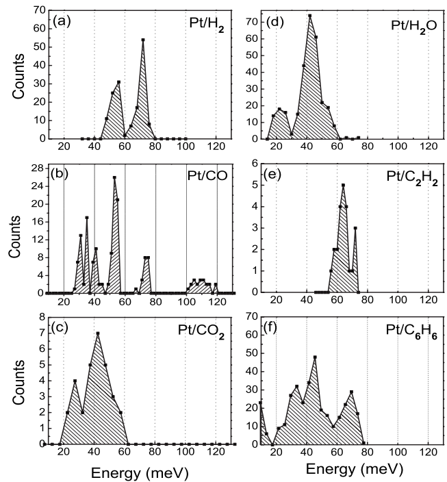
FIG. 5. Distribution of vibration-mode energies observed for (a) H_2 , (b) CO, (c) CO_2 , (d) H_2O , (e) C_2H_2 , and (f) C_6H_6 between Pt electrodes. The data was collected for junctions with zero-bias conductance below 1.1G_0 (for C_6H_6 this range is wider than appears in a previous report (Ref. 7) where the data was collected for zero-bias conductance below 0.4G_0 ). Note that for Pt/CO and Pt/ C_2H_2 junctions only a limited set of data was collected.
