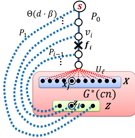
Fig. 6: Lower bound construction for (1, n^\delta) FT-ABFS structures. If less than |X||Z| \cdot n^{-\epsilon} edges are taken into the structure, there exists a pair (x_j, z_j) whose distance in G^*(cn) is increased by at least n^\delta . Consequently, when e_i \in P_0 fails, the path from s to x_j is increased by at least n^\delta compared to the real distance \text{dist}(s, x_j, G \setminus \{e_i\}) .
