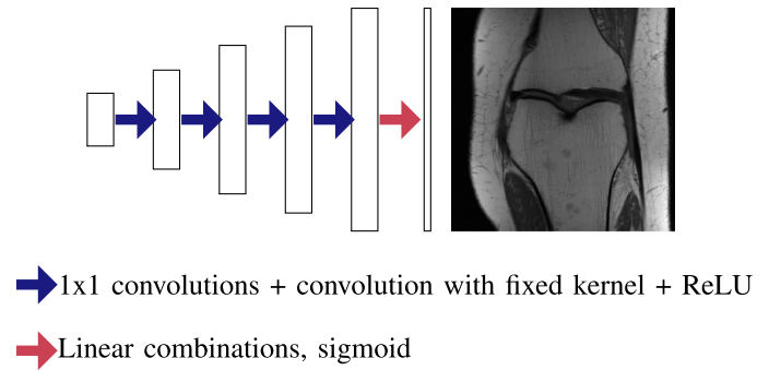
Fig. 3. A rough illustration of the deep decoder, a five-layer untrained convolutional neural network. The network performs 1 \times 1 convolutions (i.e., linear combinations of channels) followed by convolutions with a fixed kernel to map one volume to another. Convolution with a fixed kernel often includes an upsampling operation, as displayed here.
